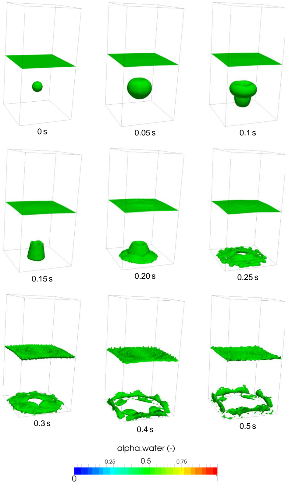
3D depth charge, alpha = 0.5 iso-surfaces, parallel simulation
